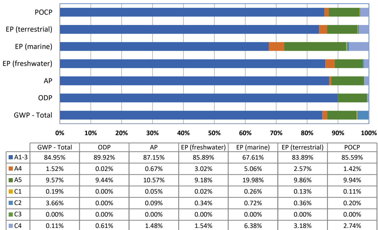
Figure 1 - shows the relative contribution of each life cycle stage to different environmental indicators for the carbon steel reinforcing bars manufactured by the secondary production route (scrap)
