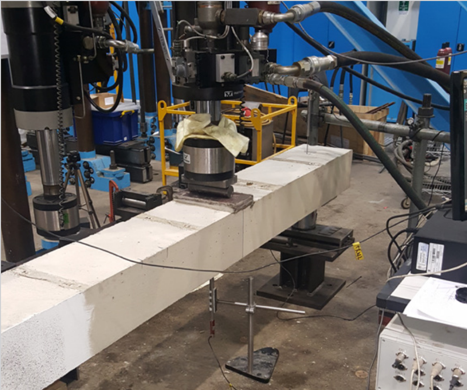
Figure 2 - Test arrangement
