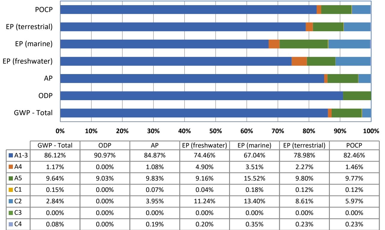
Figure 1 - shows the relative contribution of each life cycle stage to different environmental indicators for the carbon steel reinforcing bars manufactured by the secondary (scrap based) production route
