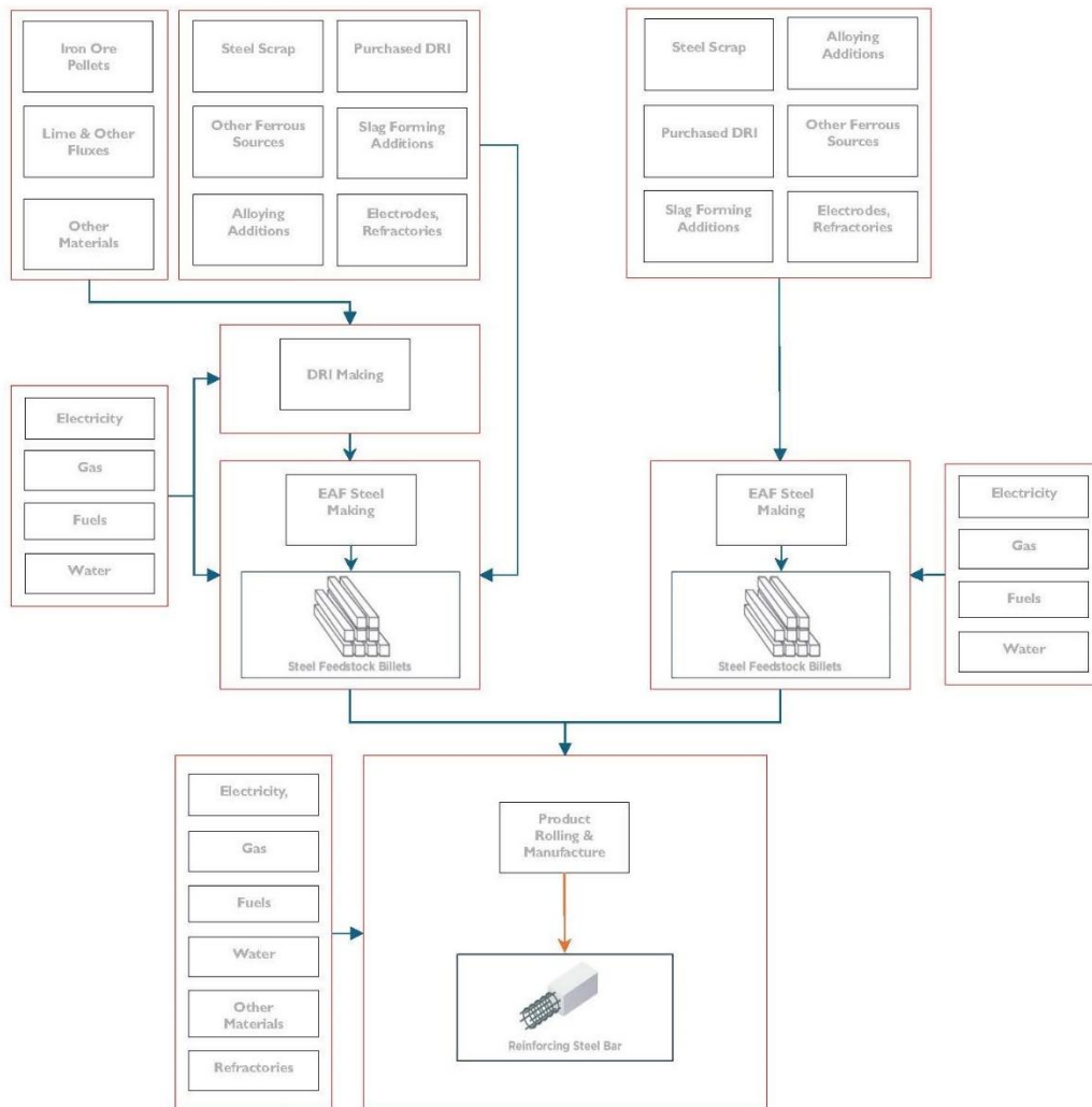
DRI/SAF and Scrap/SAF steelmaking routes and rolling
