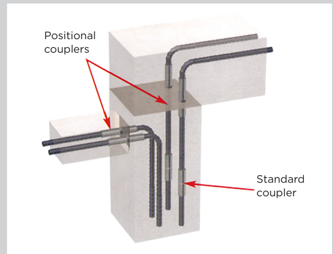
Typical application of GRIPTEC positional coupler
