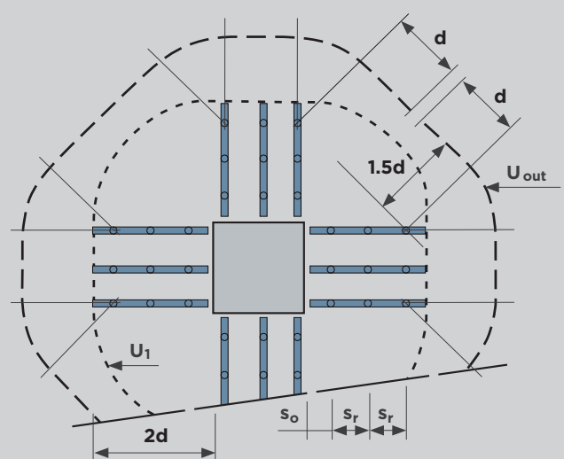
Figure 3 Detailing requirements
