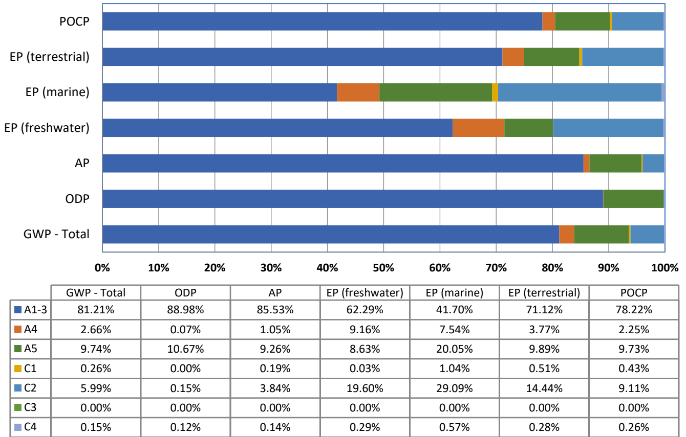
Figure 1 - shows the relative contribution of each life cycle stage to different environmental indicators for the carbon steel reinforcing bars manufactured by the secondary (scrap-based) production route
